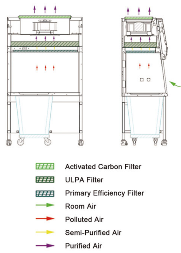
Air Flow Pattern Diagram:
